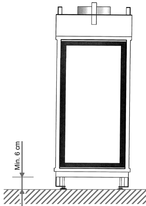
Figure 15: A clearance of at least 6 cm must be maintained between the bottom of the appliance and the floor.
